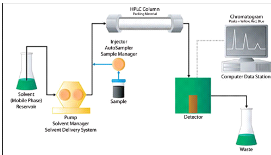
Figure 1: Block diagram of HPLC instrumentation
